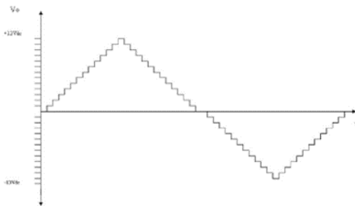
Figure 5: Typical output waveform for Hybrid H-Bridge Multilevel Inverter
