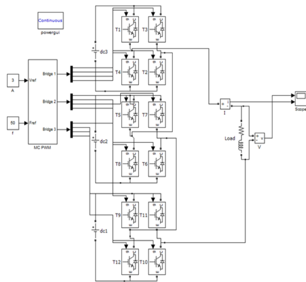
Figure 6: Simulink model for Hybrid H-Bridge Multilevel Inverter with 27 levels
