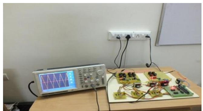
Figure 11: Hardware setup for 27 Multilevel Inverter
