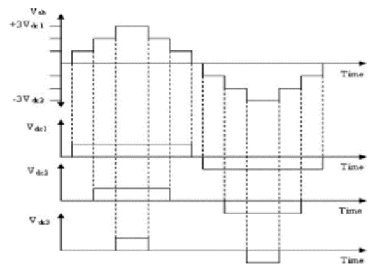
Figure 3: Typical Output Waveform for Cascaded H-Bridge Multilevel Inverter
