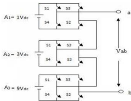
Figure 4: Hybrid H-Bridge Multilevel Inverter
