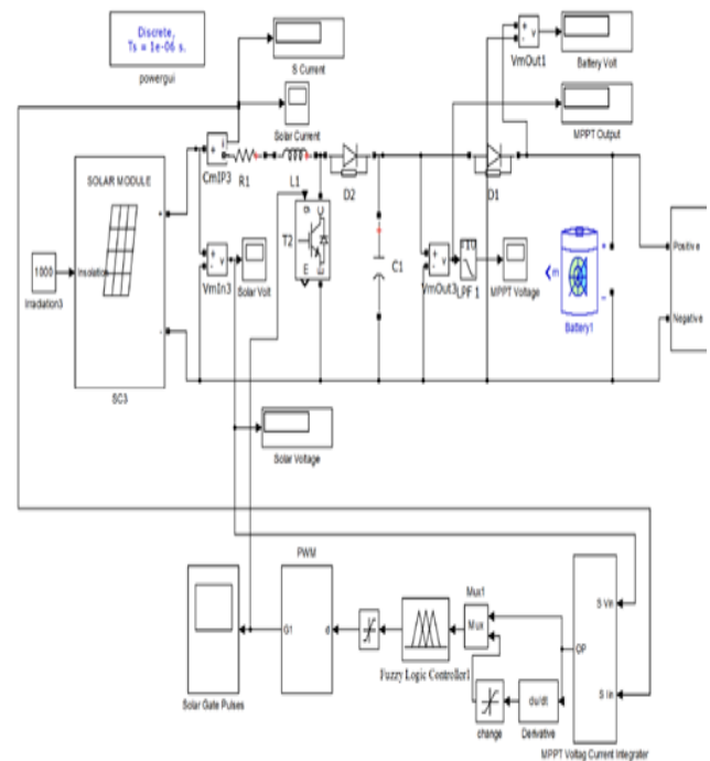
Figure 5: Simulink model for PV system using MPPT technique
