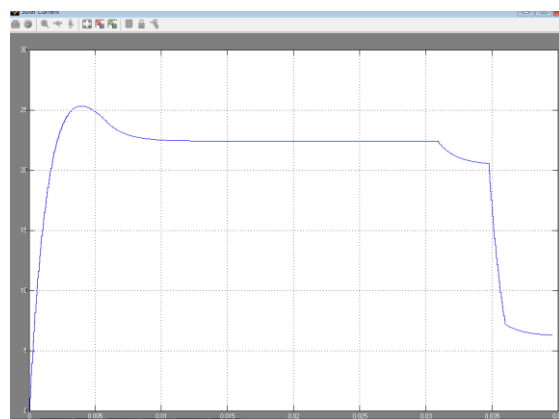
Figure 7: Output of Solar Current
